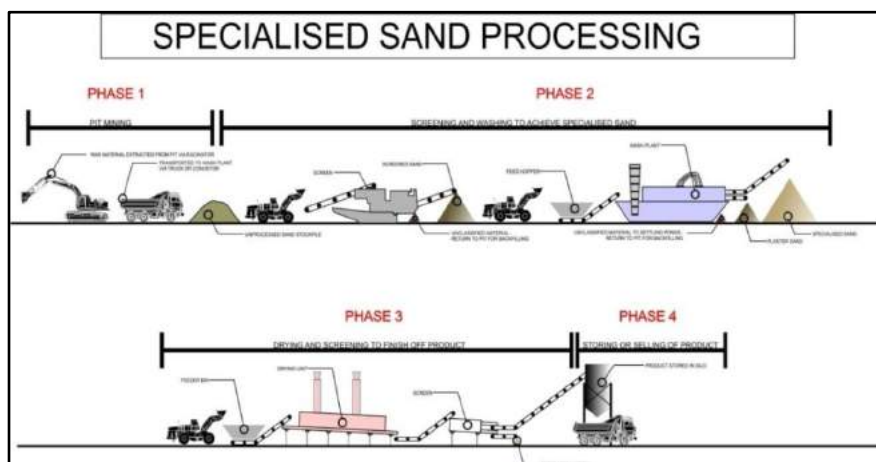
Figure 2: Specialised sand processing.
