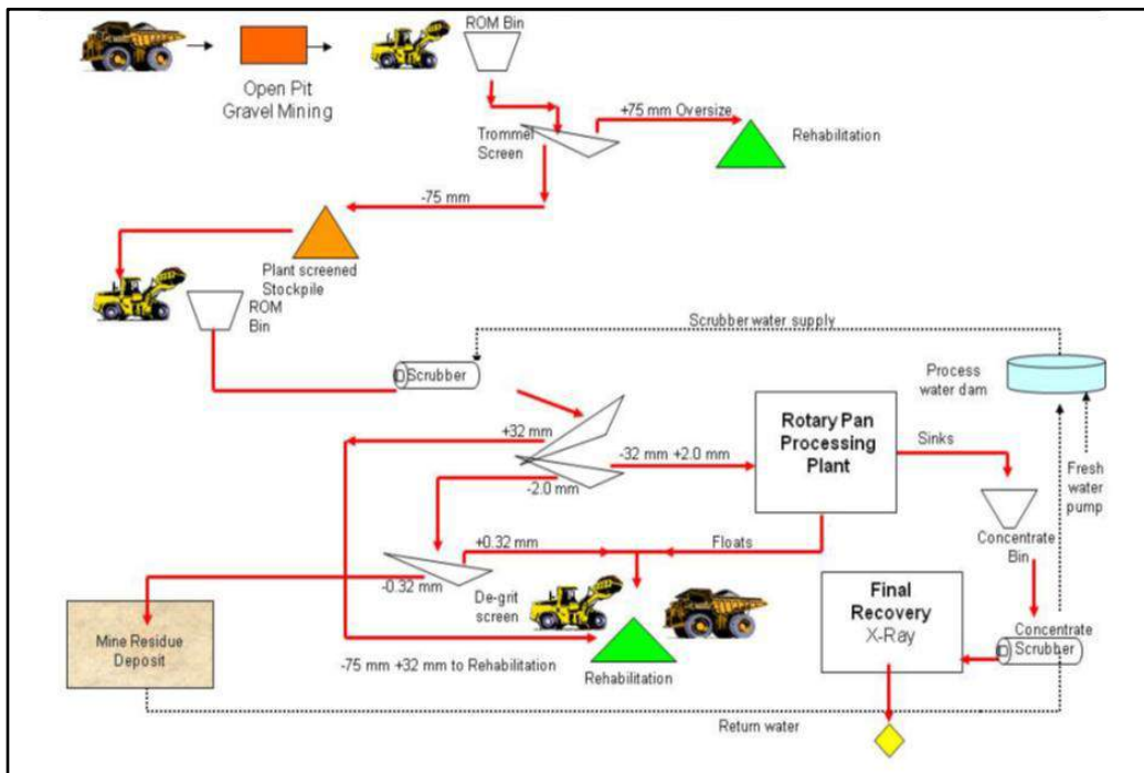
Figure 4: Diamond extraction methodology.
