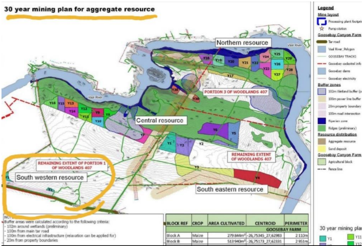
30 Year Mine Plan for Aggregate - South Western Resource
