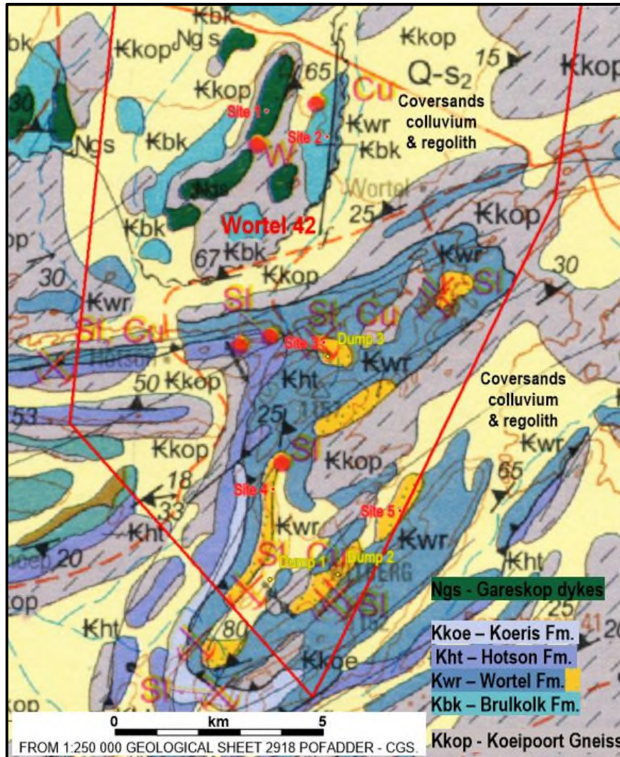
Figure 2. Geology of the Project Area, with drilling and dump sampling sites indicated.
