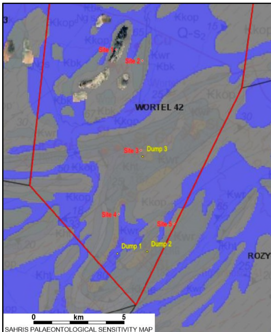
Figure 5. Palaeontological sensitivity of the Project Area. Grey – no palaeontological studies required. Blue - no palaeontological studies required, but a protocol for fossil finds is required. The clear patches (e.g. Site 1) are unfossiliferous outcrops of the Gareskop intrusions.
